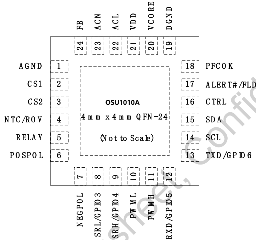
Figure 2 OSU1010A-AA000-QN24R Pin Assignment
