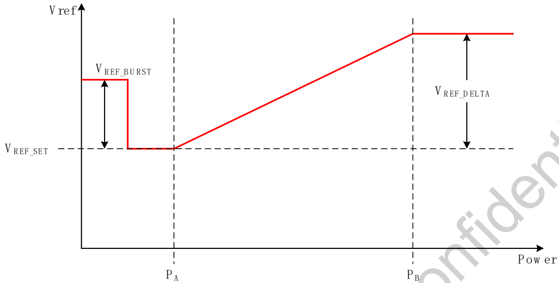
Figure 9 Bus Voltage Adaptive Adjustment Based on Power
