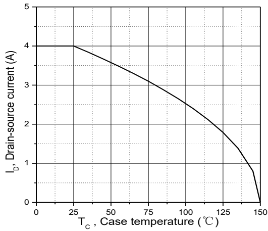
Figure 9. Drain current
