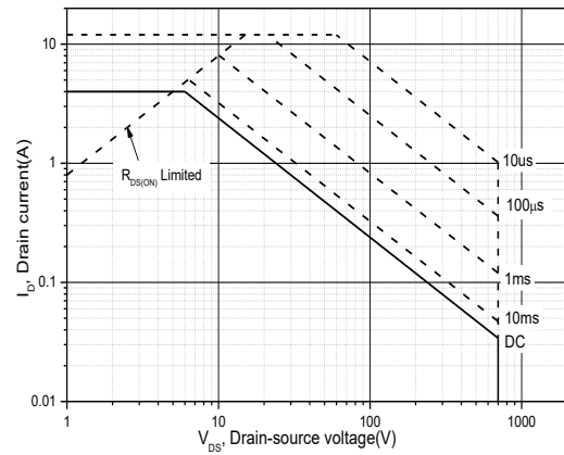
Figure 10. Safe operation area Tc=25 °C
