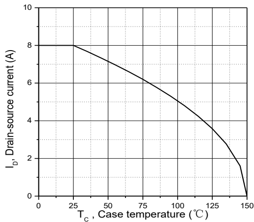
Figure 9. Drain current
