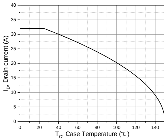
Figure 9. Drain current
