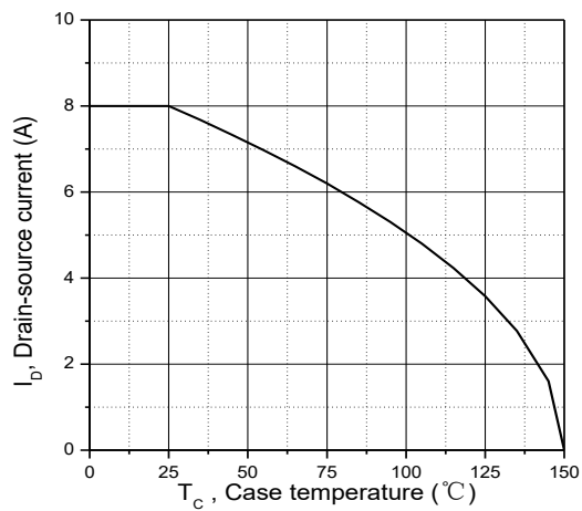
Figure 9. Drain current
