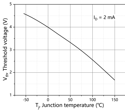
Figure 7. Threshold voltage
