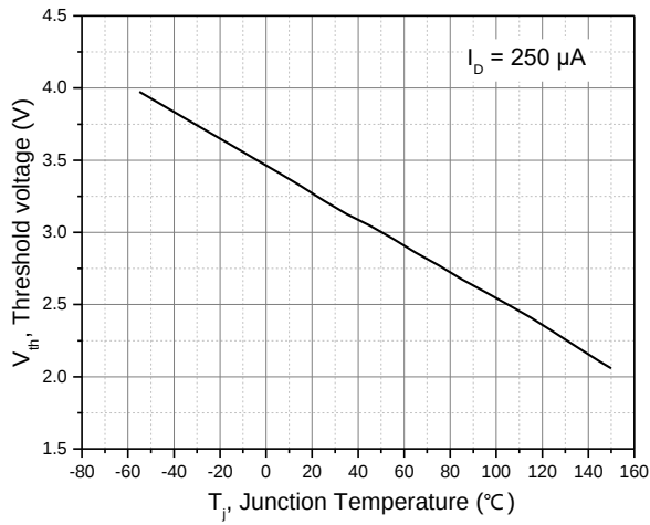
Figure 7. Threshold voltage
