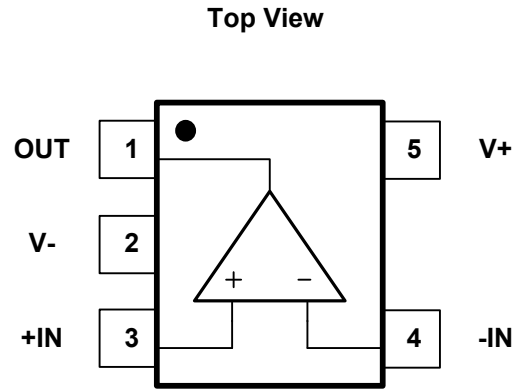
Fig.5-2. OSU6721B: S5 (SOT23-5) Package
