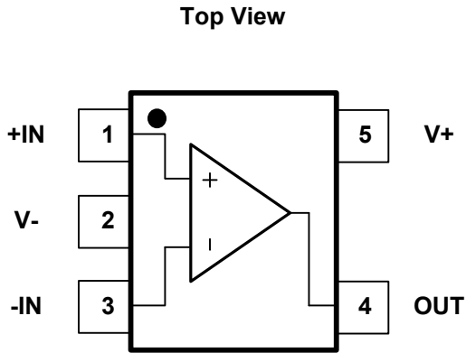
Fig.5-1. OSU6721: C5 (SC70-5) Package OSU6721: S5 (SOT23-5) Package
