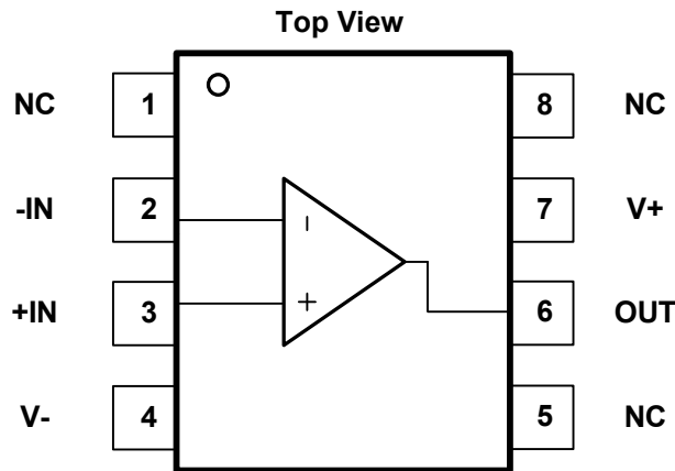
Fig.5-3. OSU6051: M8(MSOP8) Package
