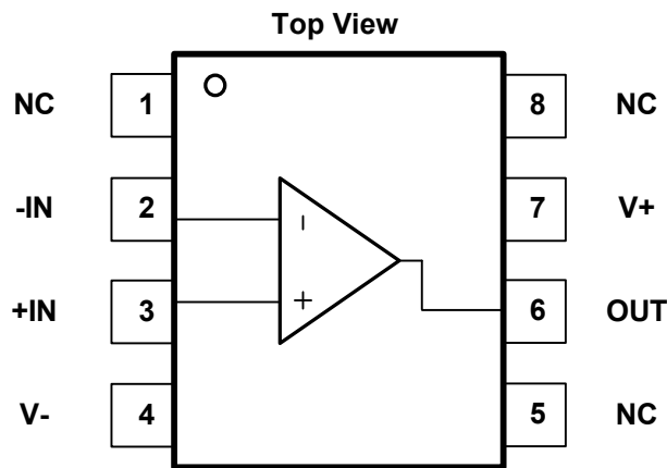
Fig.5-3. OSU6021: M8(MSOP8) Package OSU6021: P8(SOP8) Package
