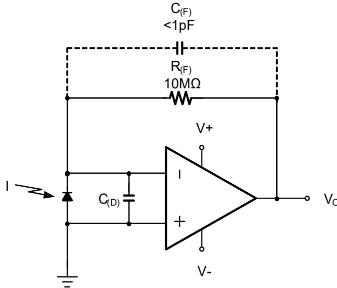
Fig.10-1. Dual-Supply Amplifier
