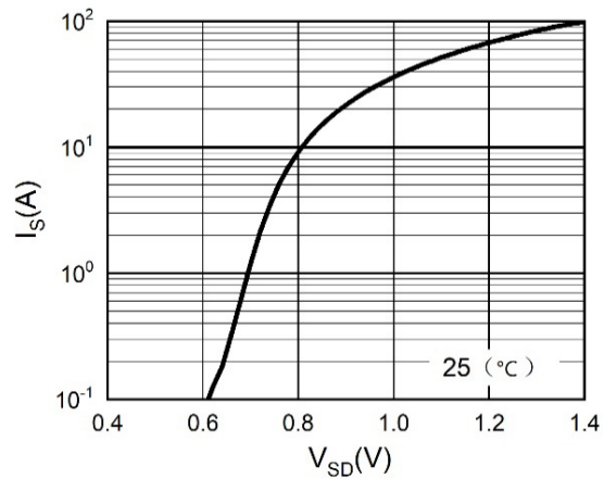
Figure 3. Body-diode Characteristics
