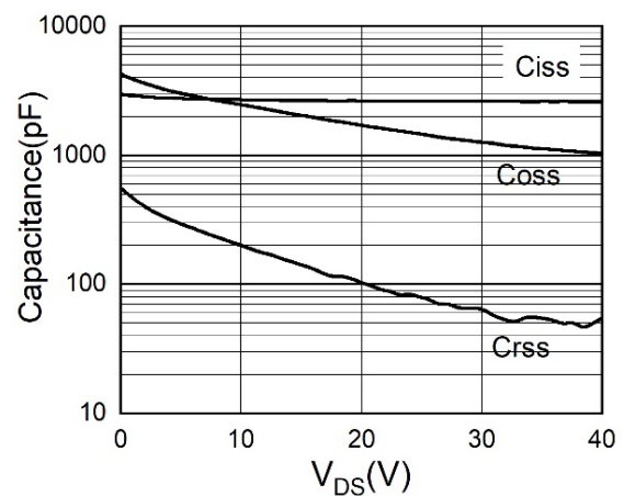
Figure 6. Capacitance
