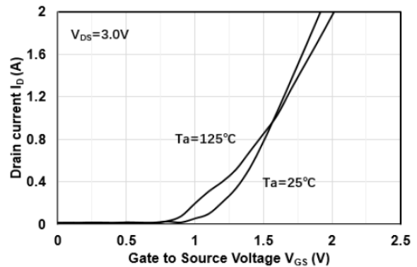
Figure 2. Typ. transfer characteristics
