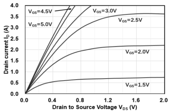
Figure 1. Typ. output characteristics
