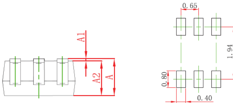
SOT-363 Suggested Pad Layout
