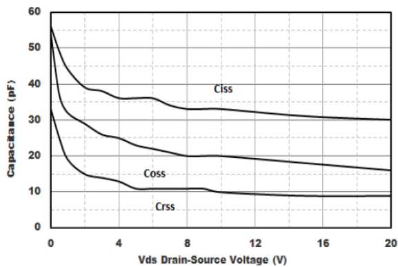
Figure 3. Typ. capacitances
