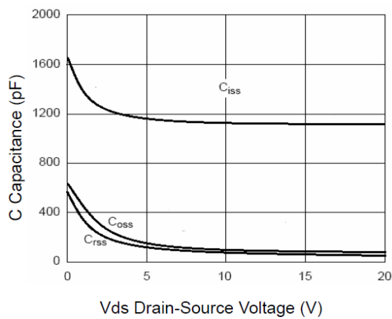
Figure 3. Capacitance
