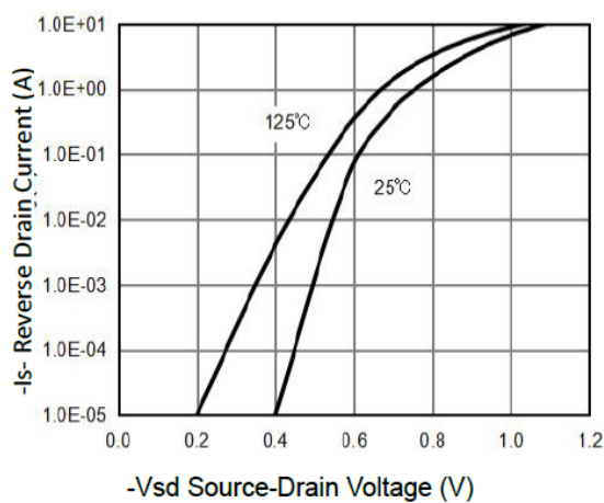
Figure 5. Body-diode characteristics
