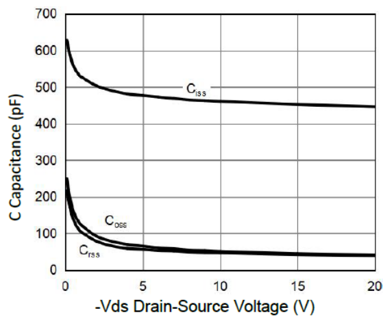
Figure 3. Capacitance
