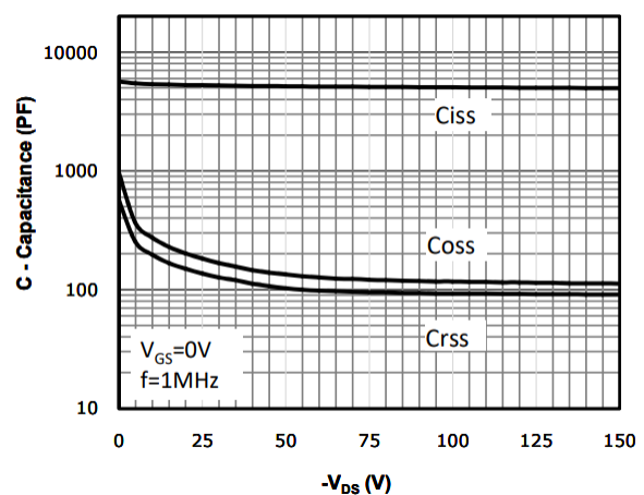
Figure 6. Capacitance
