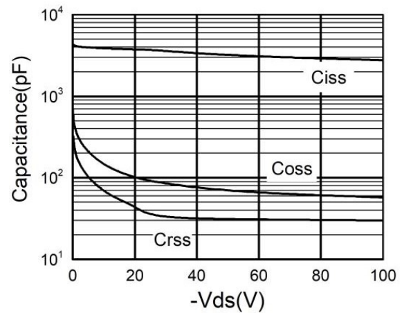
Figure 6. Capacitance
