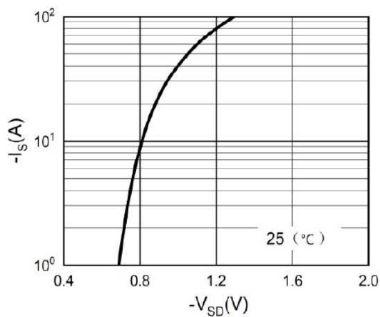
Figure 3. Body-diode characteristics
