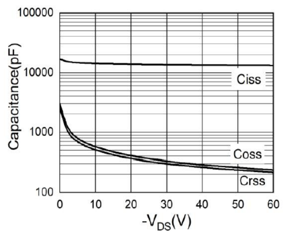
Figure 6. Capacitance
