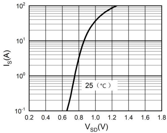
Figure 3. Body-diode characteristics
