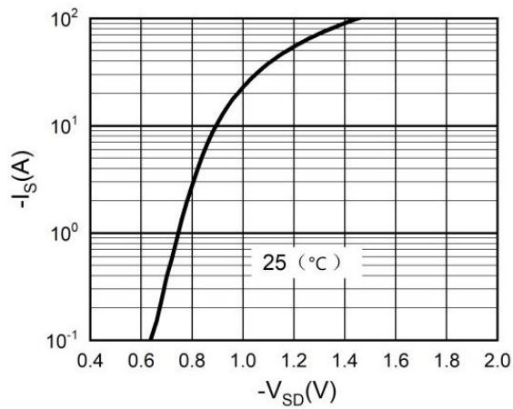
Figure 3. Body-diode characteristics
