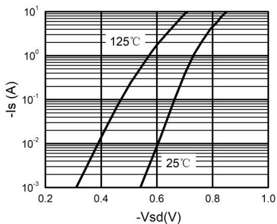
Figure 5. Body-diode characteristics
