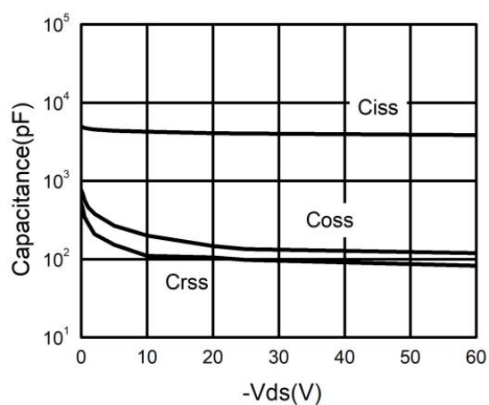
Figure 4. Capacitance
