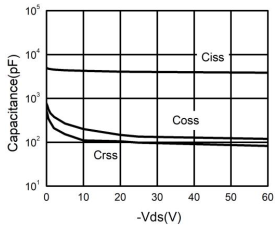
Figure 4. Capacitance
