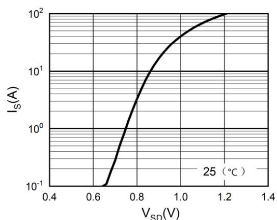
Figure 5. Body-diode characteristics
