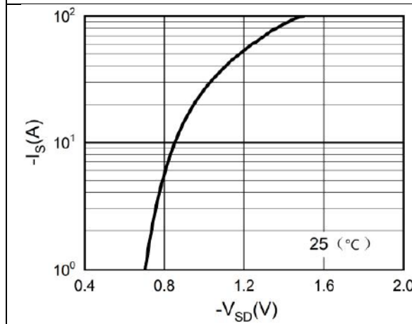
Figure 3. Body-diode characteristics
