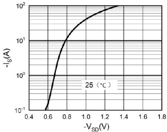
Figure 3. Body-diode characteristics
