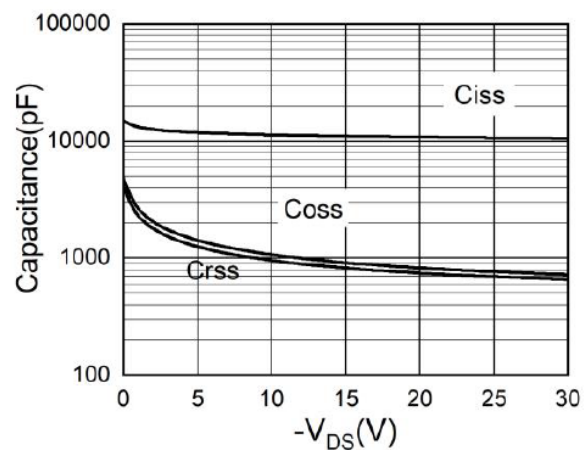
Figure 6. Capacitance
