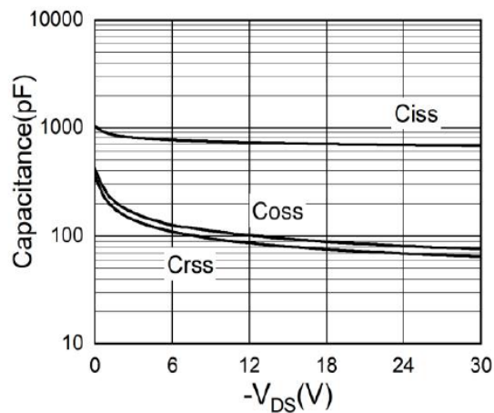
Figure 3. Capacitance
