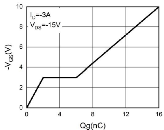
Figure 4. Gate charge
