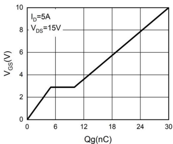
Figure 5. Gate charge waveforms
