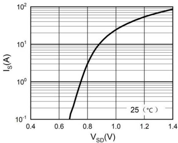
Figure 3. Body-diode characteristics
