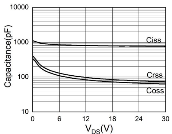
Figure 6. Capacitance
