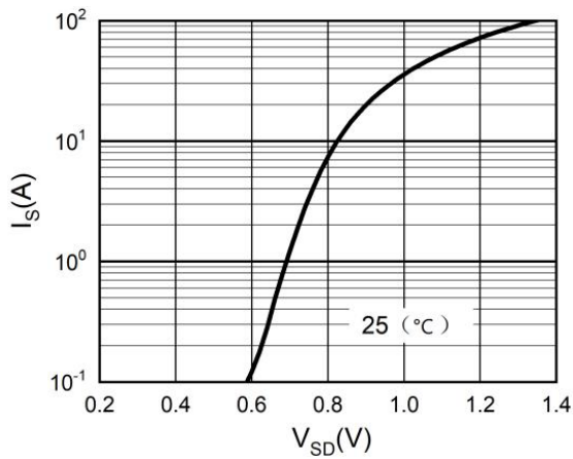
Figure 3. Body-diode characteristics
