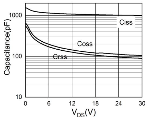
Figure 6. Capacitance
