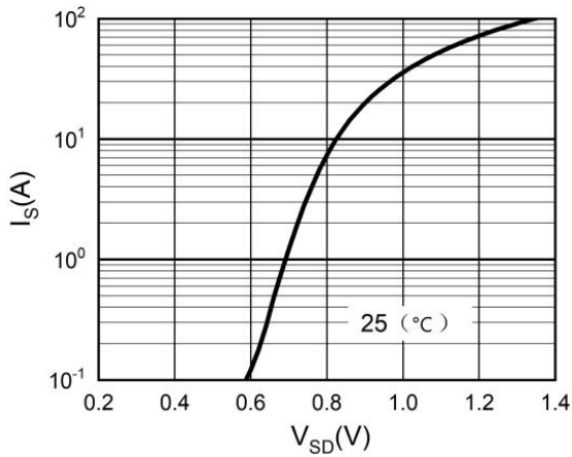
Figure 3. Body-diode characteristics
