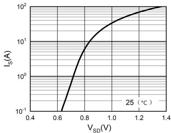
Figure 5. Body-diode characteristics
