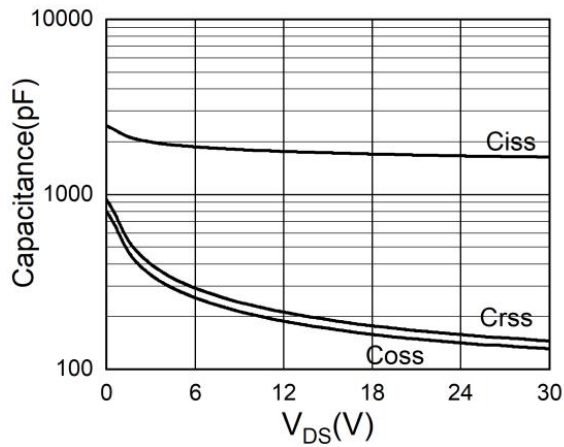
Figure 3. Capacitances
