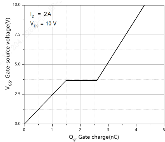
Figure 4. Gate charge
