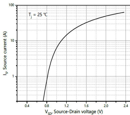
Figure 5. Body-diode characteristics
