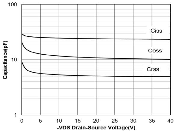
Figure 3. Typ. capacitances
