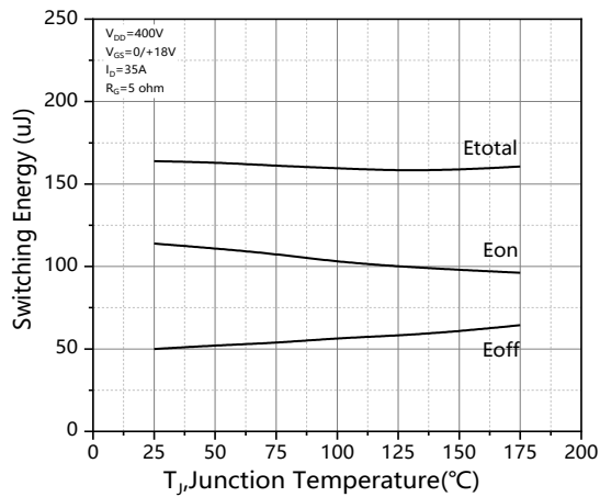
Figure 21. Clamped inductive switching energy vs. temperature
