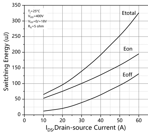
Figure 19. Clamped inductive switching energy vs. drain current
