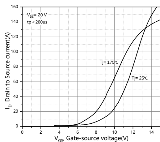
Figure 6. Transfer characteristic for various junction temperatures
