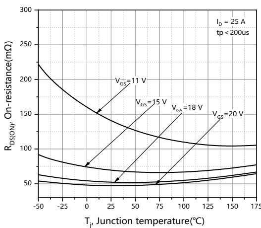
Figure 5. On-resistance vs. temperature for various gate voltage
