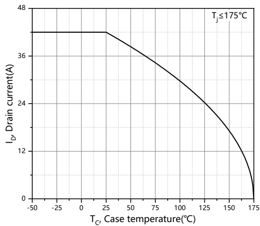
Figure 15. Continuous drain current derating vs. case temperature
