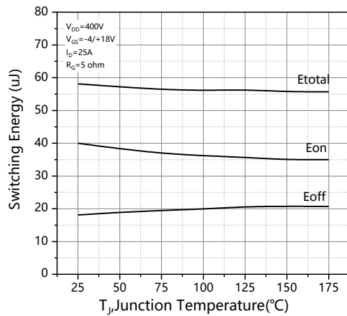
Figure 21. Clamped inductive switching energy vs. temperature
