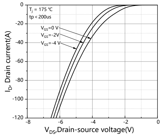
Figure 8. Body diode characteristic at T_j = 175\text{ °C}
