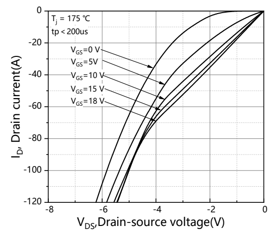
Figure 12. 3rd quadrant characteristic at T_j = 175\text{ °C}
