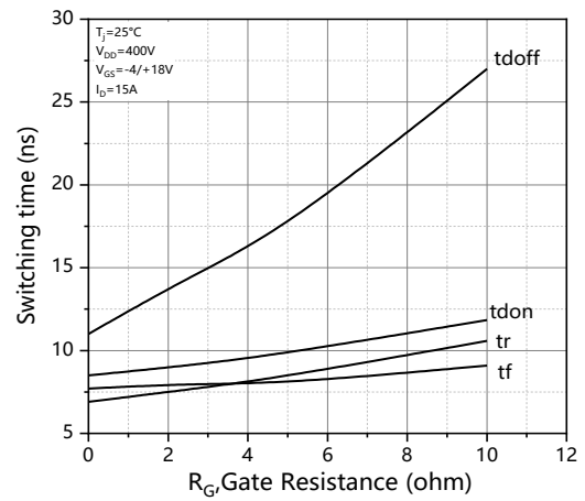
Figure 22. Switching times vs. R_G
