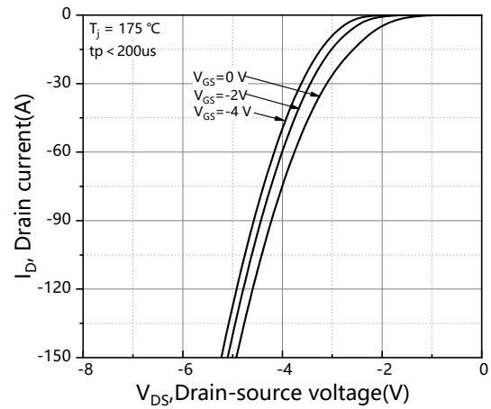
Figure 8. Body diode characteristic at T_j = 175\text{ }^{\circ}\text{C}
