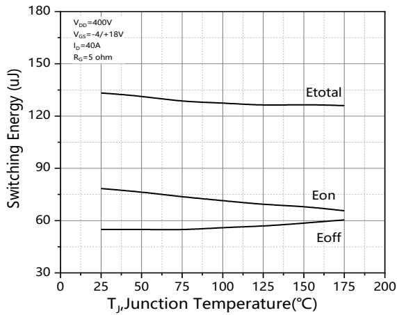
Figure 21. Clamped inductive switching energy vs. temperature
