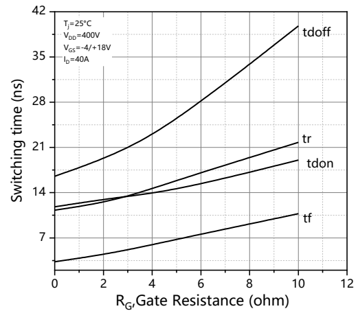
Figure 22. Switching times vs. R_G
