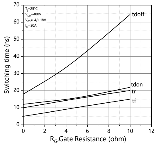
Figure 22. Switching times vs. R_G
