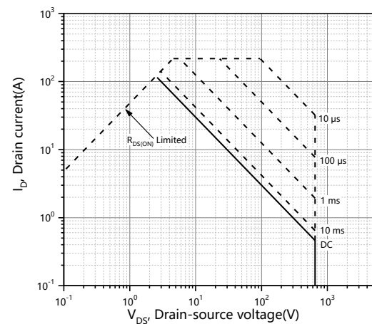
Figure 18. Safe operating area
