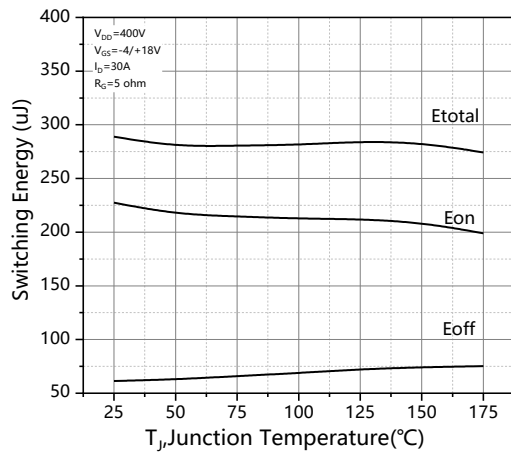
Figure 21. Clamped inductive switching energy vs. temperature
