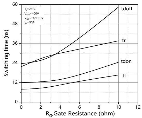
Figure 22. Switching times vs. R_G
