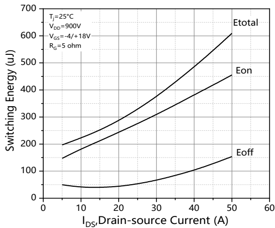
Figure 21. Clamped inductive switching energy vs. drain current ( V_{DD} = 900V )
