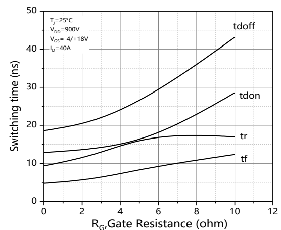
Figure 24. Switching times vs. R_G
