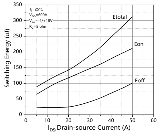
Figure 20. Clamped Inductive switching energy vs. drain current ( V_{DD} = 600V )
