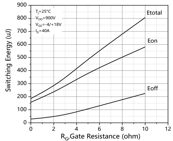
Figure 22. Clamped inductive switching energy vs. R_G
