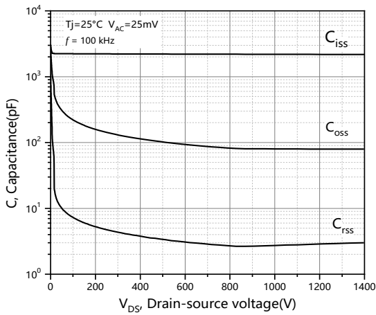
Figure 15. Capacitances vs. drain-source voltage (0 - 1400V)
