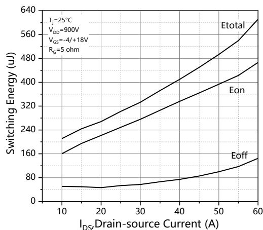
Figure 21. Clamped inductive switching energy vs. drain current ( V_{DD} = 900V )
