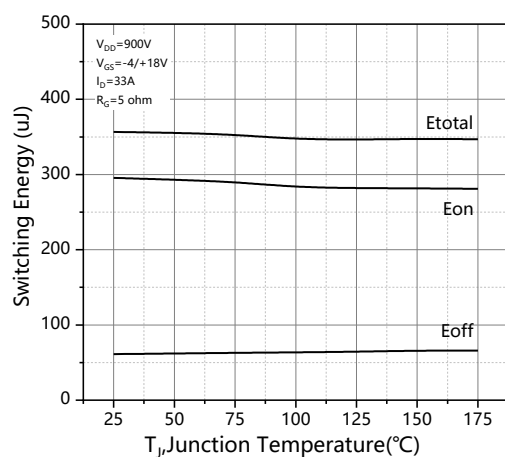
Figure 23. Clamped inductive switching energy vs. temperature
