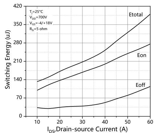
Figure 20. Clamped Inductive switching energy vs. drain current ( V_{DD} = 700V )
