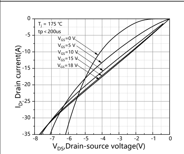
Figure 12. 3rd quadrant characteristic at T_j = 175\text{ °C}
