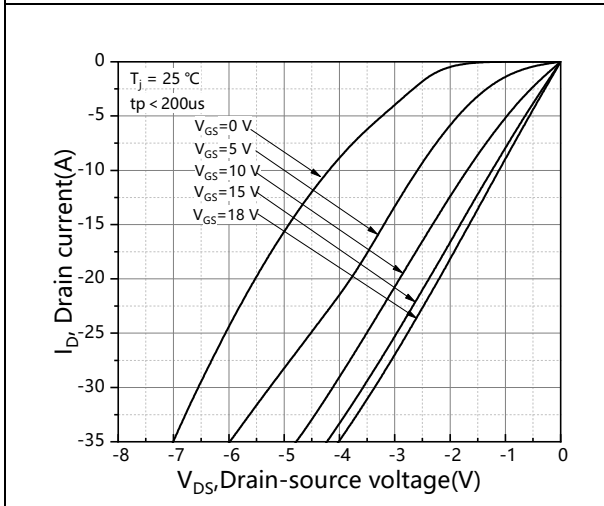
Figure 11. 3rd quadrant characteristic at T_j = 25\text{ °C}
