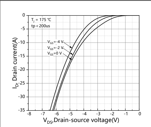
Figure 8. Body diode characteristic at T_j = 175\text{ °C}
