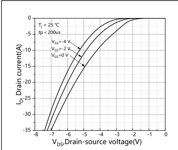
Figure 7. Body diode characteristic at T_j = 25\text{ °C}
