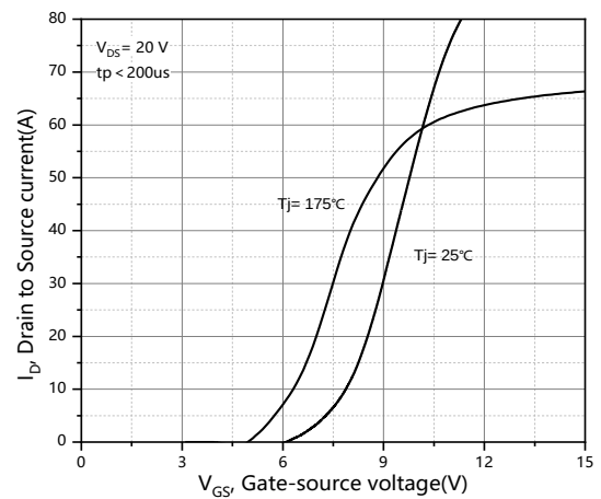
Figure 6. Transfer characteristic for various junction temperatures
