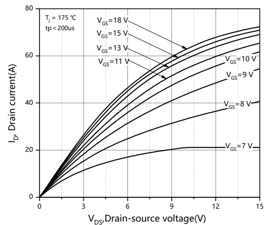
Figure 2. Output characteristics T_j=175\text{ °C}
