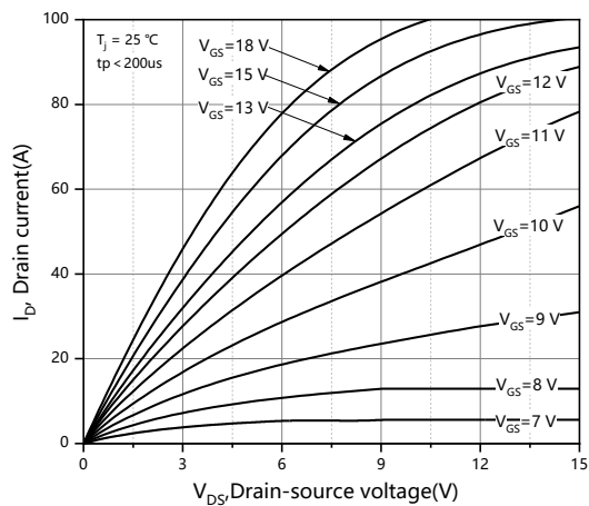
Figure 1. Output characteristics T_j=25\text{ °C}
