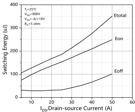
Figure 21. Clamped inductive switching energy vs. drain current ( V_{DD} = 800V )
