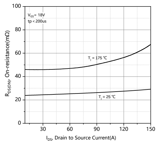
Figure 4. On-resistance vs. drain current for various temperatures
