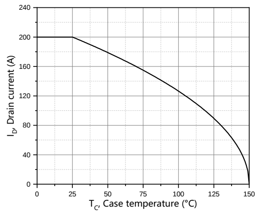
Figure 10. Drain current
