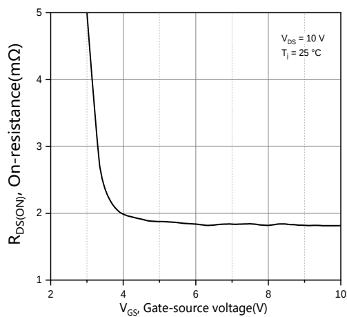
Figure 13. On-Resistance VS. Gate to Source Voltage
