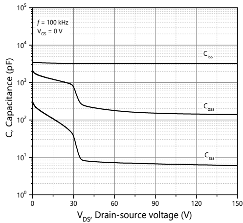
Figure 3. Typ. capacitances
