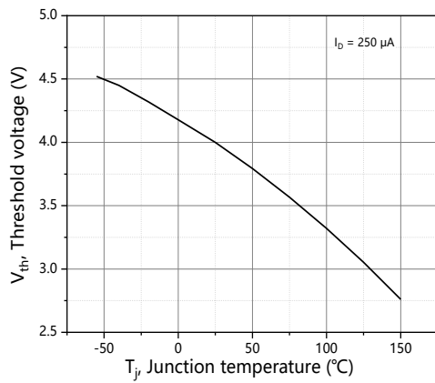
Figure 7. Threshold voltage
